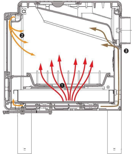
Illustration 4: air flow control
